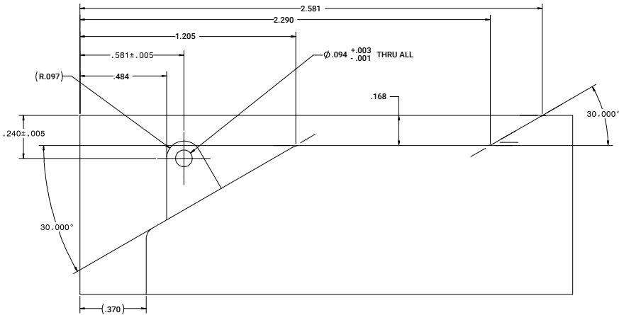
For VITA 48.2 Primary Side Configuration 1. Shown 2. Opposite
