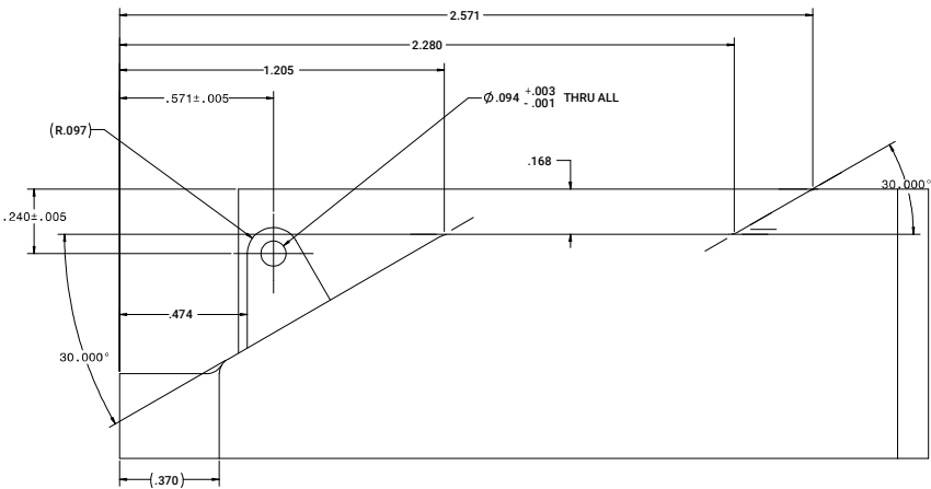
For VITA 48.2 Secondary Side Configuration 1. Shown 2. Opposite
