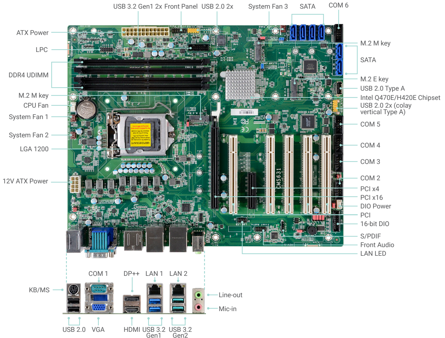
Top View (CMS631-Q470E)
