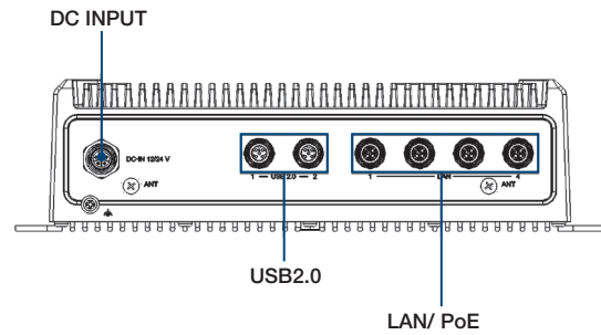
Rear Panel
