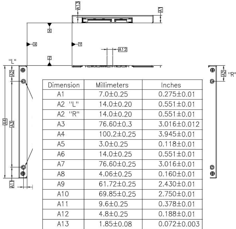
Figure 2-1. 2.5" SSD Dimensions
