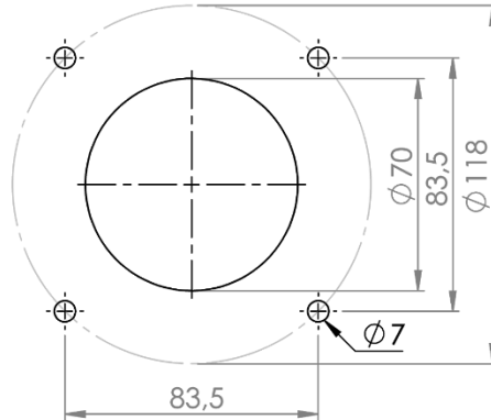
Mounting Cut-Out Enclosure Ø130 mm
