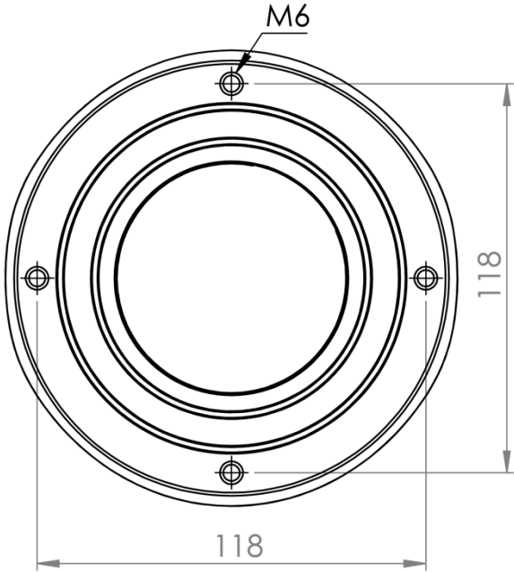
Floor Connection Dimension
