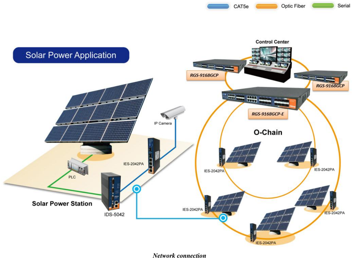
Network connection
