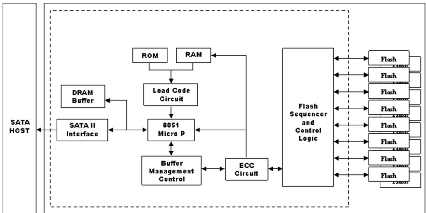
Figure 1: APRO SLC Industrial 2.5" SATA III SSD HERMES-HR Series block diagram
