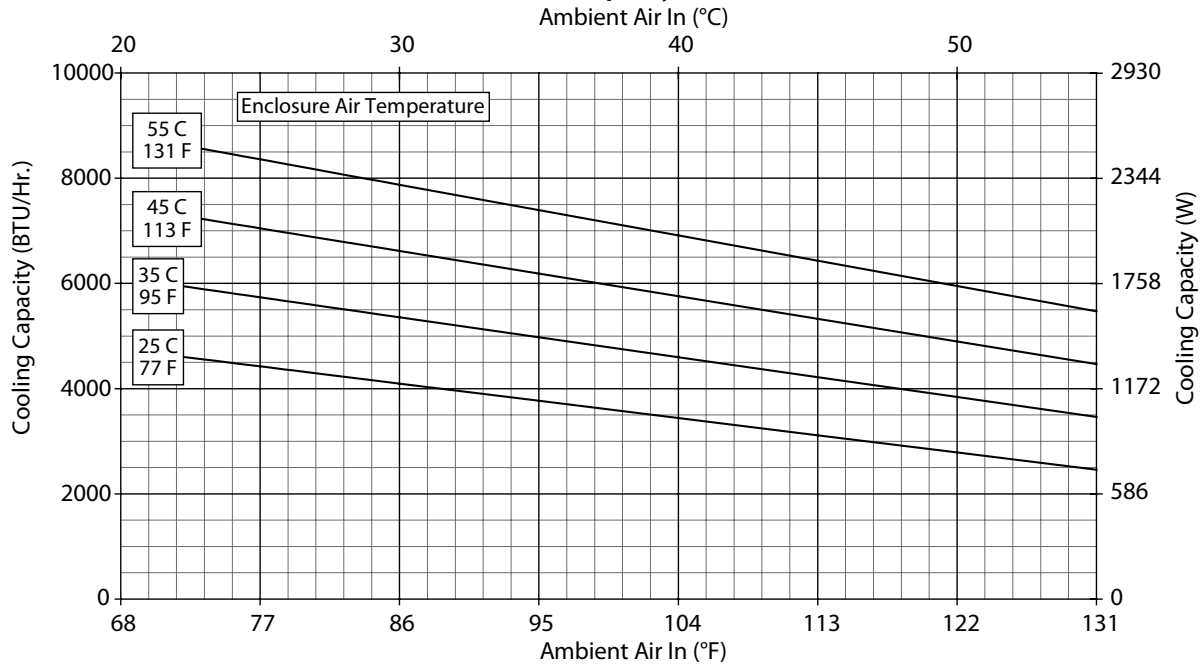
N36-0626-GXXX Capacity Curves at 50 Hz
