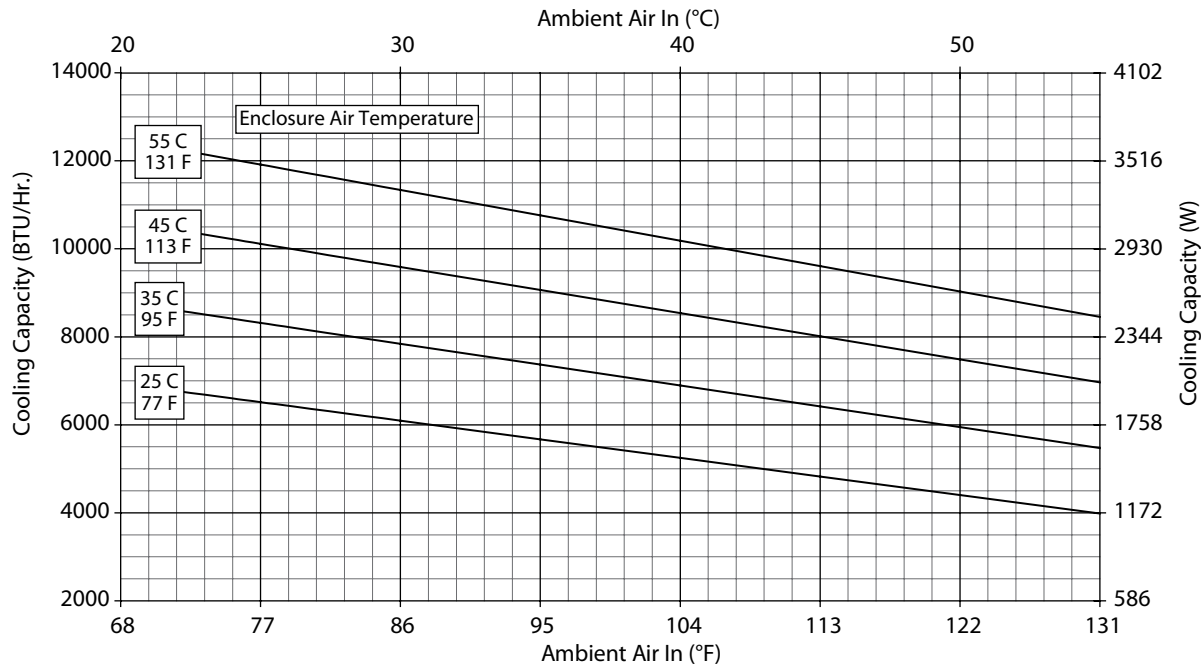
N36-0816-GXXX Capacity Curves at 60 Hz
