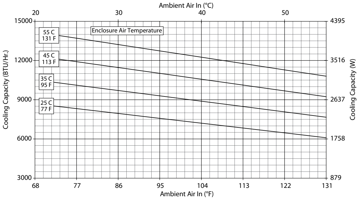
N43-1246-GXXX Capacity Curves at 60 Hz
