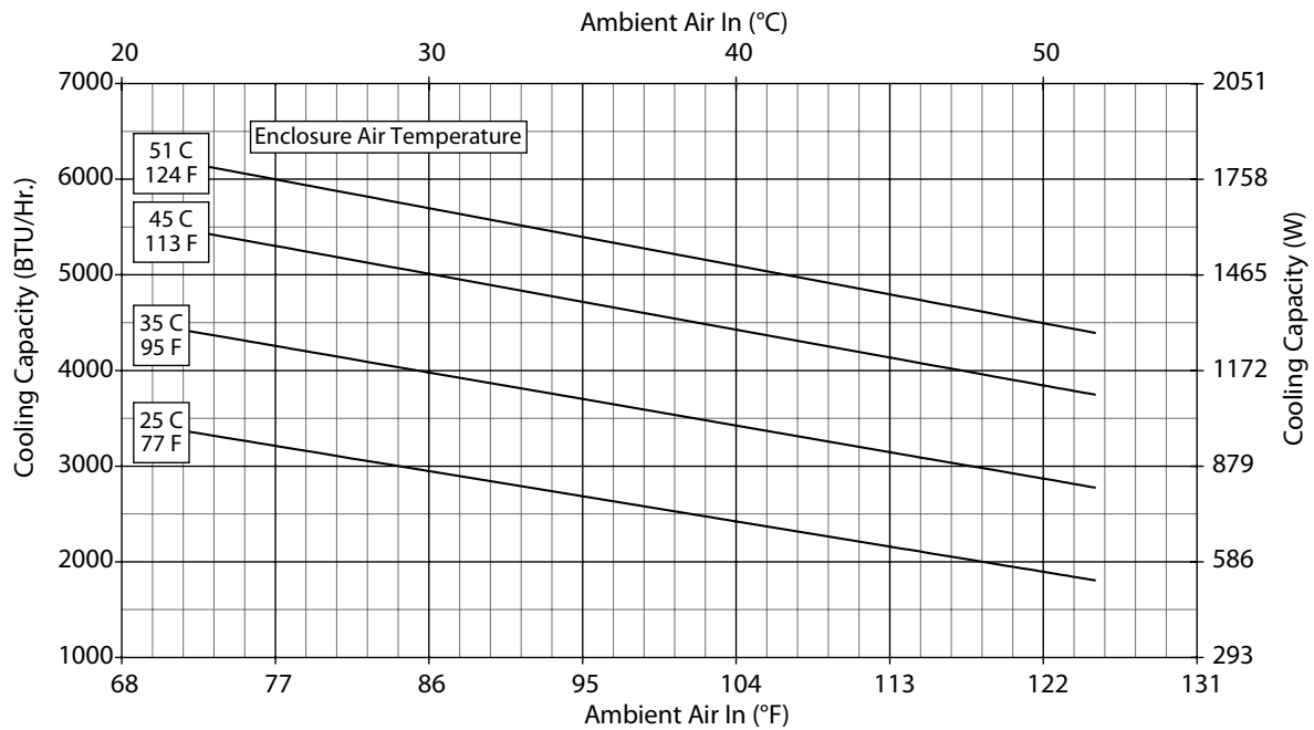
N28-0426-GXXX Capacity Curves at 60 Hz
