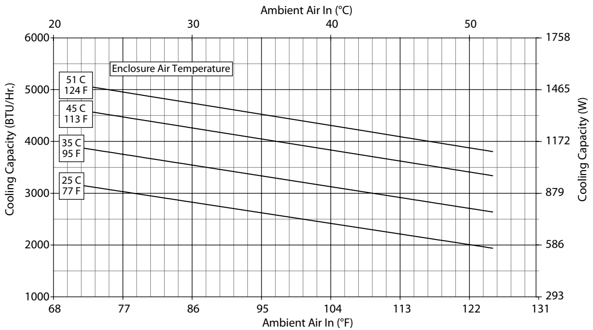
N28-0416-GXXX Capacity Curves at 50 Hz
