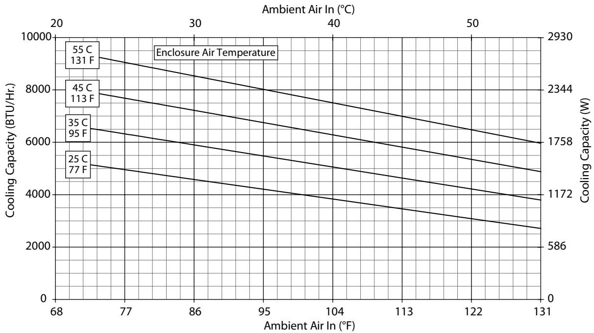
N36-0626-GXXX Capacity Curves at 60 Hz
