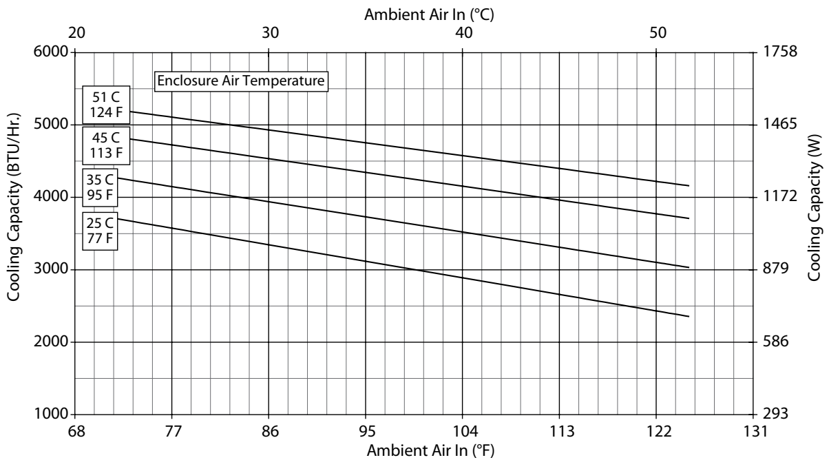
N28-0416-GXXX Capacity Curves at 60 Hz
