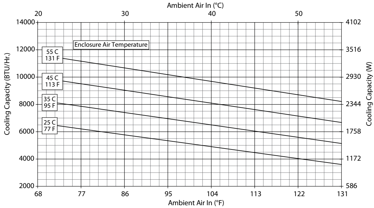
N36-0816-GXXX Capacity Curves at 50 Hz
