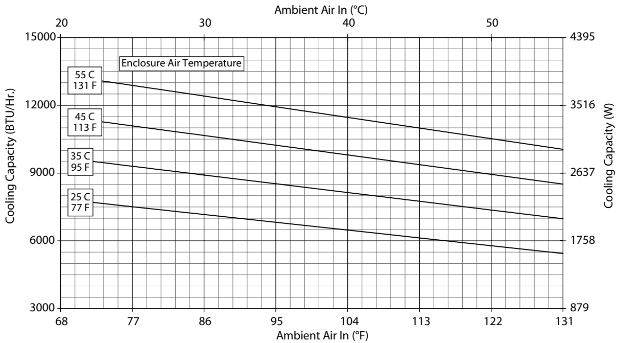
N43-1246-GXXX Capacity Curves at 50 Hz
