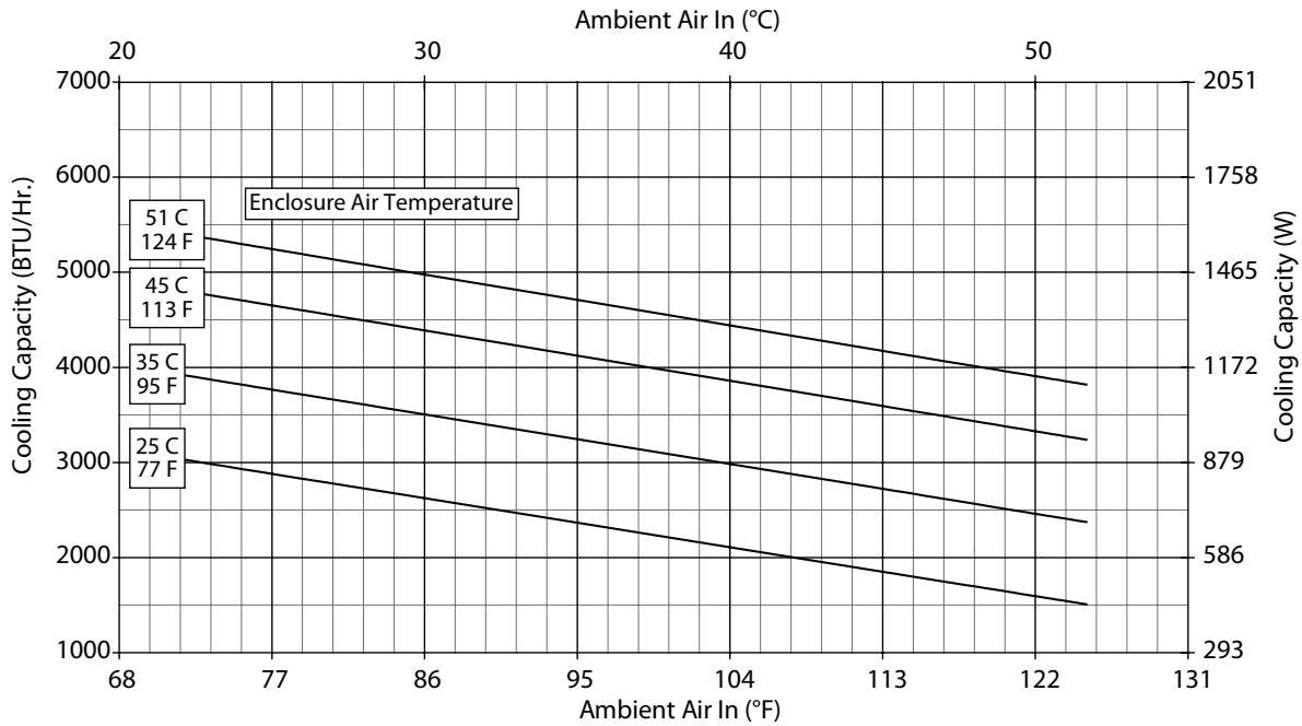
N28-0426-GXXX Capacity Curves at 50 Hz
