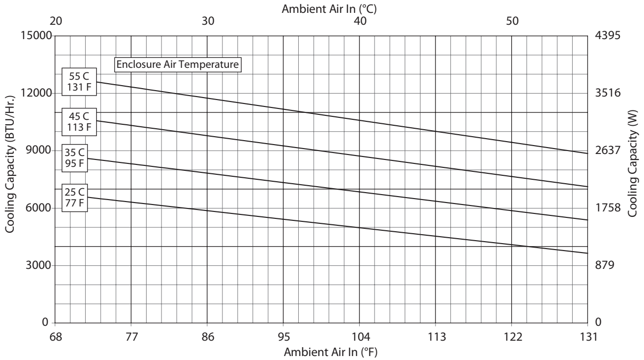
G52-0846-GXXX Capacity Curve 50 Hz
