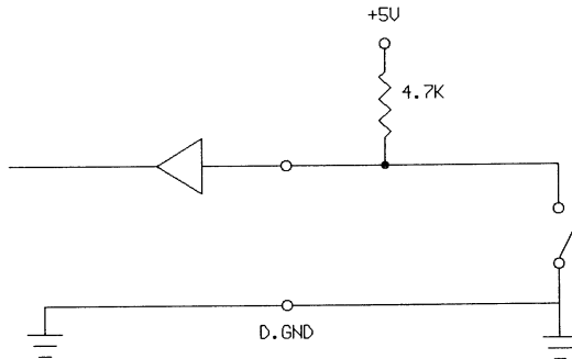
OPEN/SHORT Signal Connection
