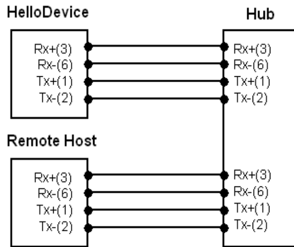
Figure A-3 Ethernet connection using straight through Ethernet cable
