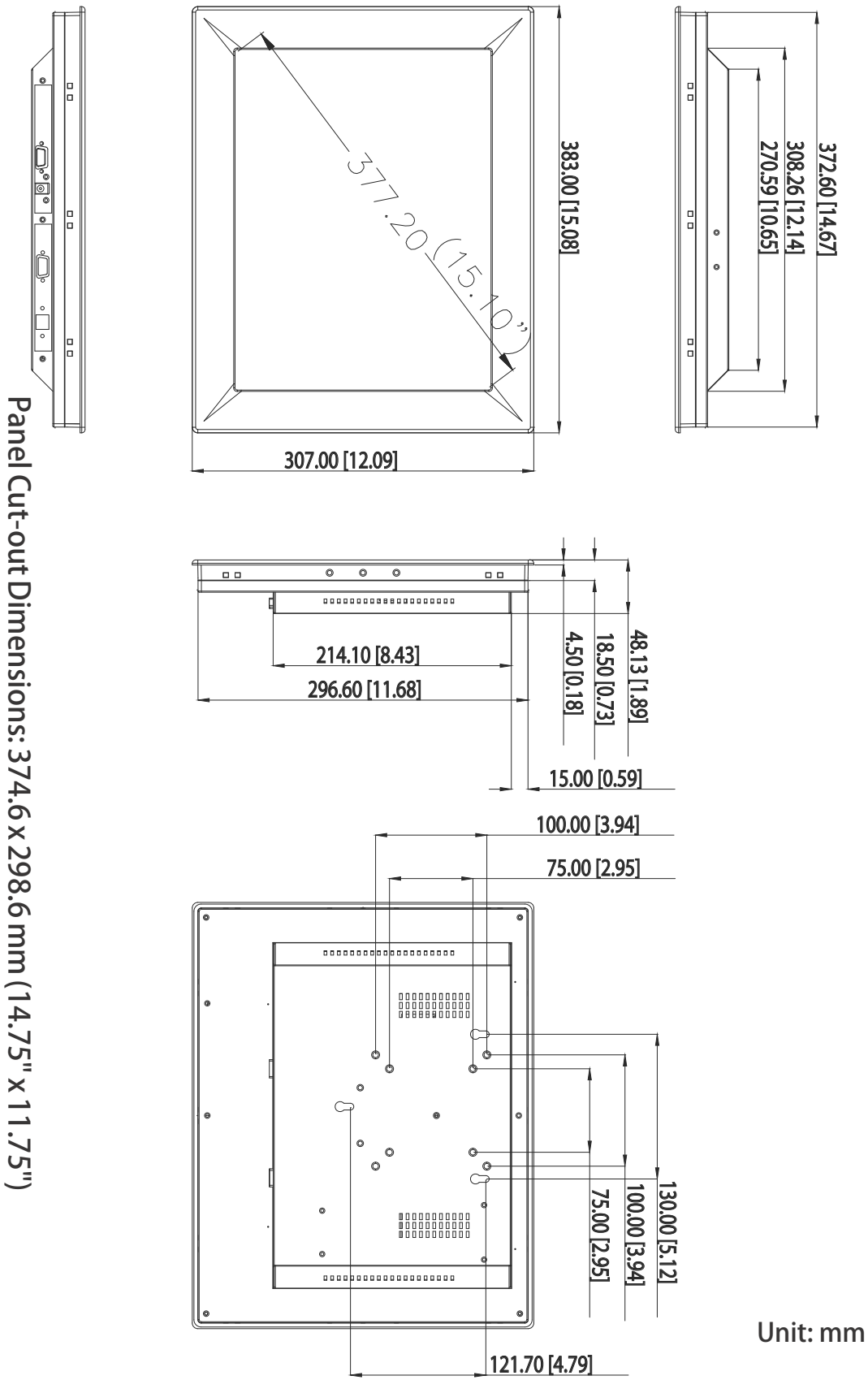
Figure 1.2 FPM-2150G Dimensions
