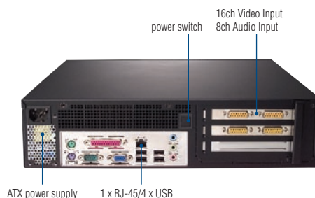
The Rear view of PVS-500
