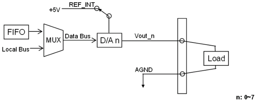
Figure 3.3: Analog Output Connections
