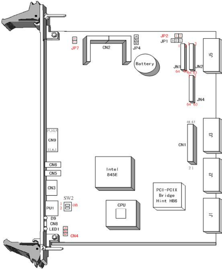
Figure 1.3: MIC-3358 jumpers and connectors
