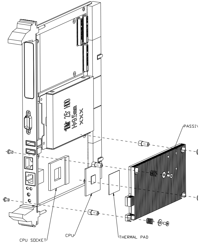
Figure 1.5: Complete assembly
