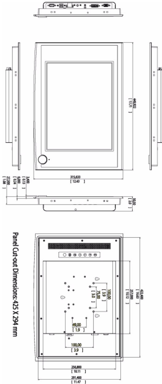
Figure 1.1: FPM-5151G Dimensions
