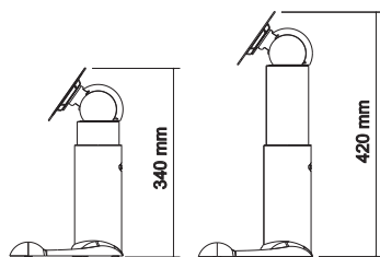
Adjust display height over a range of 80 mm for improved desktop ergonomics
