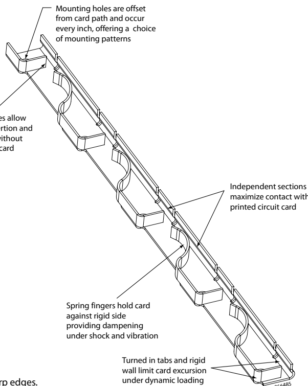
Series 125/126/165/166 retainers
